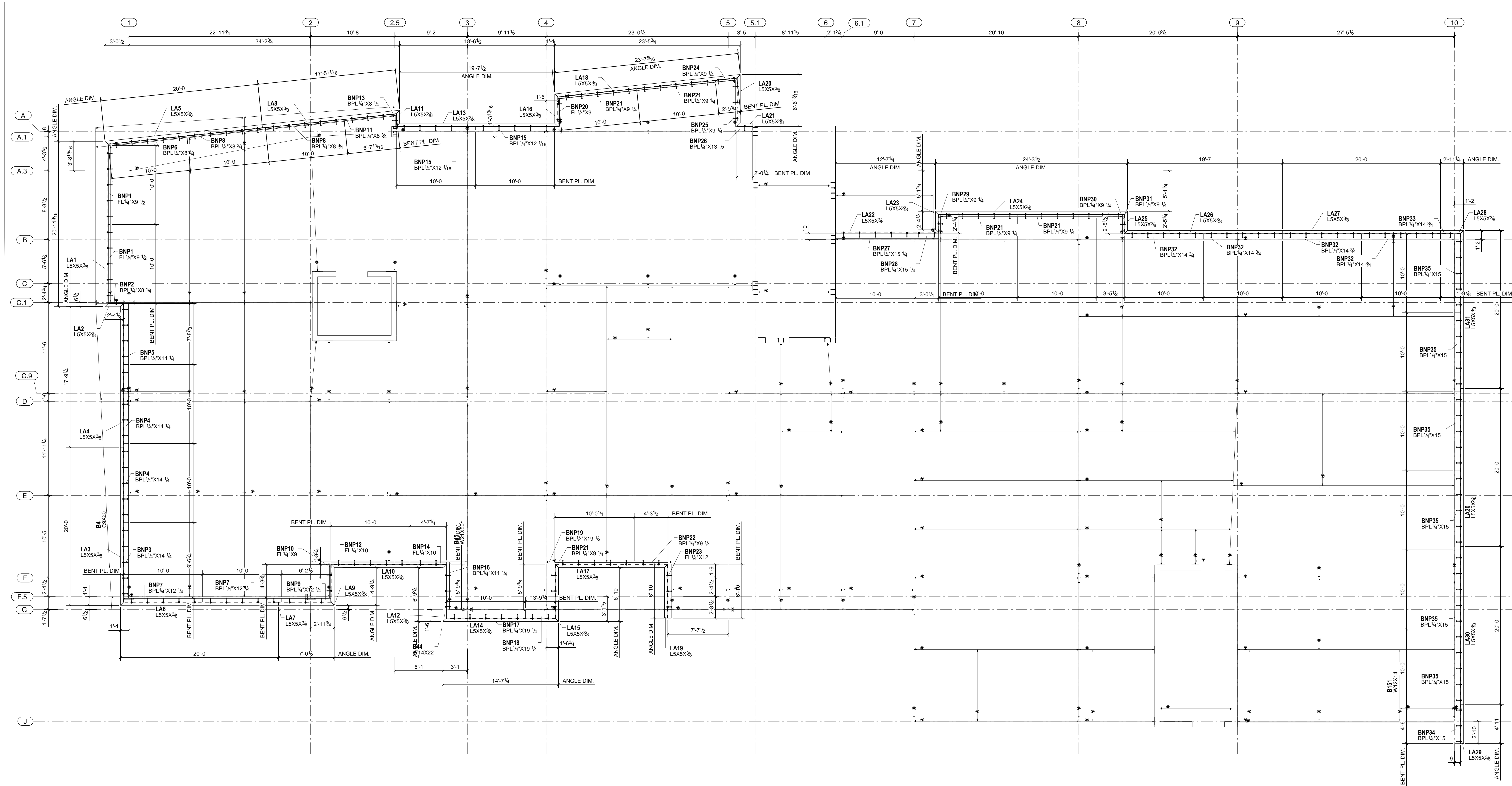
LEVEL 2 LOOSE ANGLE & BENT PLATE PLAN
