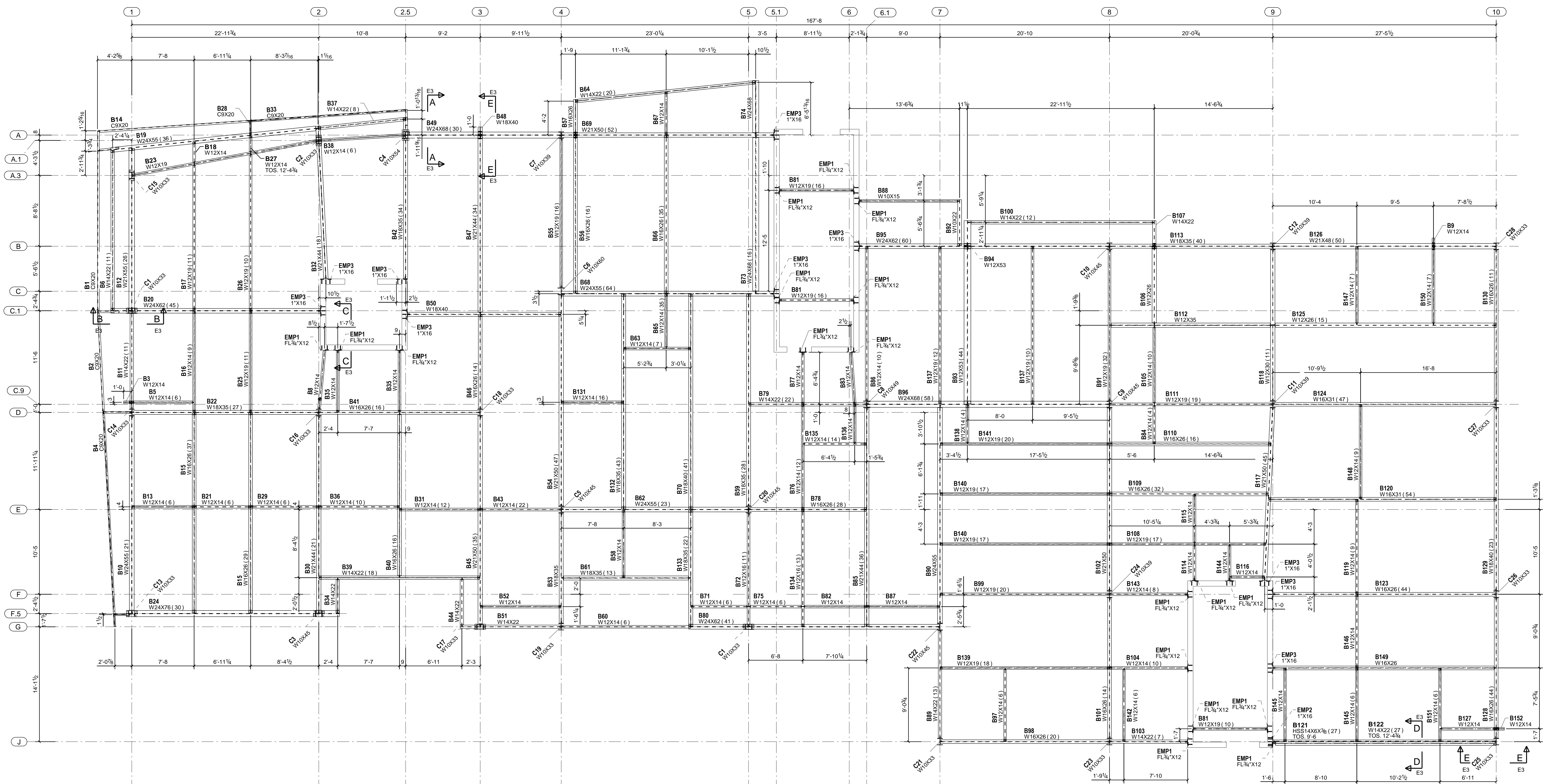
LEVEL 2 FRAMING PLAN T.O.S = 12'4 3/4"
